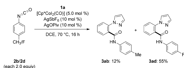
Scheme 5. Mechanistic studies.
